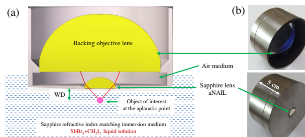
Fig. 5. (a) Schematic of the design for simultaneous increase of NA and WD, using a sapphire-based aNAIL lens system immersed in the refractive index matching liquid (solution of \text{SbBr}_3 in \text{CH}_2\text{I}_2 ). (b) Picture of an aNAIL and backing objective lens system, designed to have \text{NA} = 1.17 and \text{WD} = 12 \text{ mm} .
