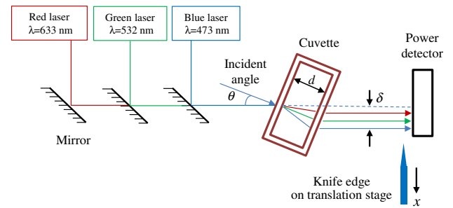
Fig. 1. Schematic of the liquid refractometer setup, based on the design of Nemoto [12]. The cuvette cross section is 20 mm \times 10 mm, with optical measurements performed across the width d = 10 mm.
