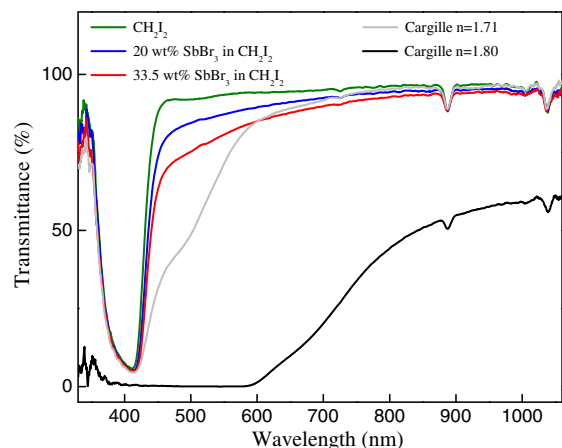
Fig. 4. Transmittance as a function of wavelength for a cuvette of width d = 10 mm.
